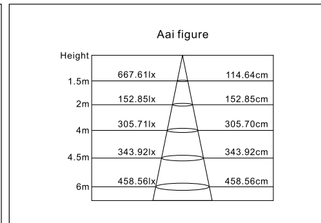
Light Distance Curve
