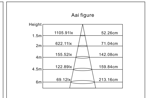
Light Distance Curve
